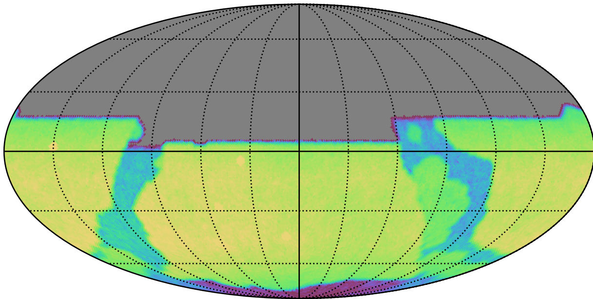
noroll_mjdp120_v3.4_10yrs All sky y band: CoaddM5
