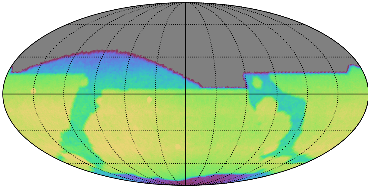
noroll_mjdp120_v3.4_10yrs All sky r band: CoaddM5
