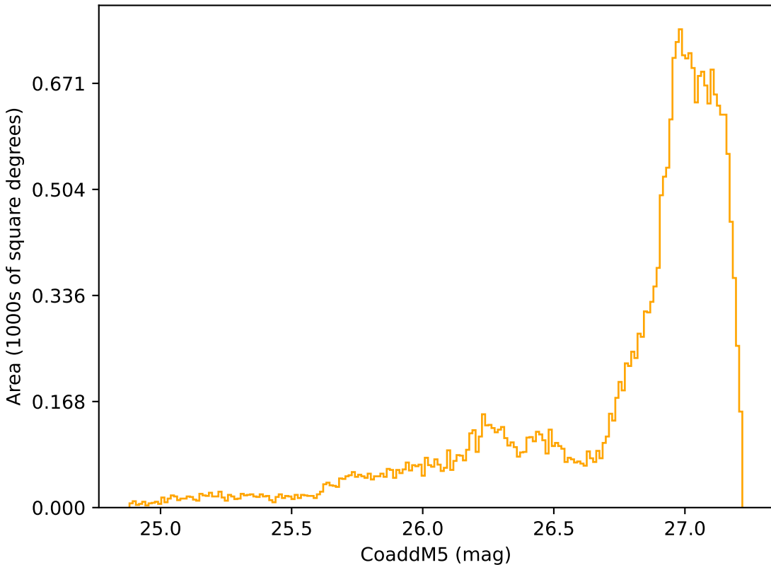
noroll_mjdp120_v3.4_10yrs All sky r band: CoaddM5
