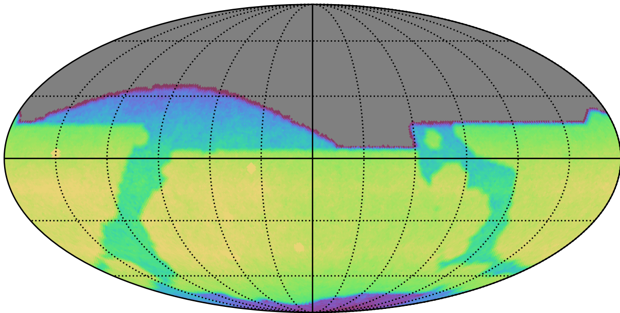
noroll_mjdp120_v3.4_10yrs All sky i band: CoaddM5
