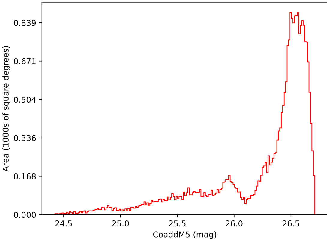
noroll_mjdp120_v3.4_10yrs All sky i band: CoaddM5
