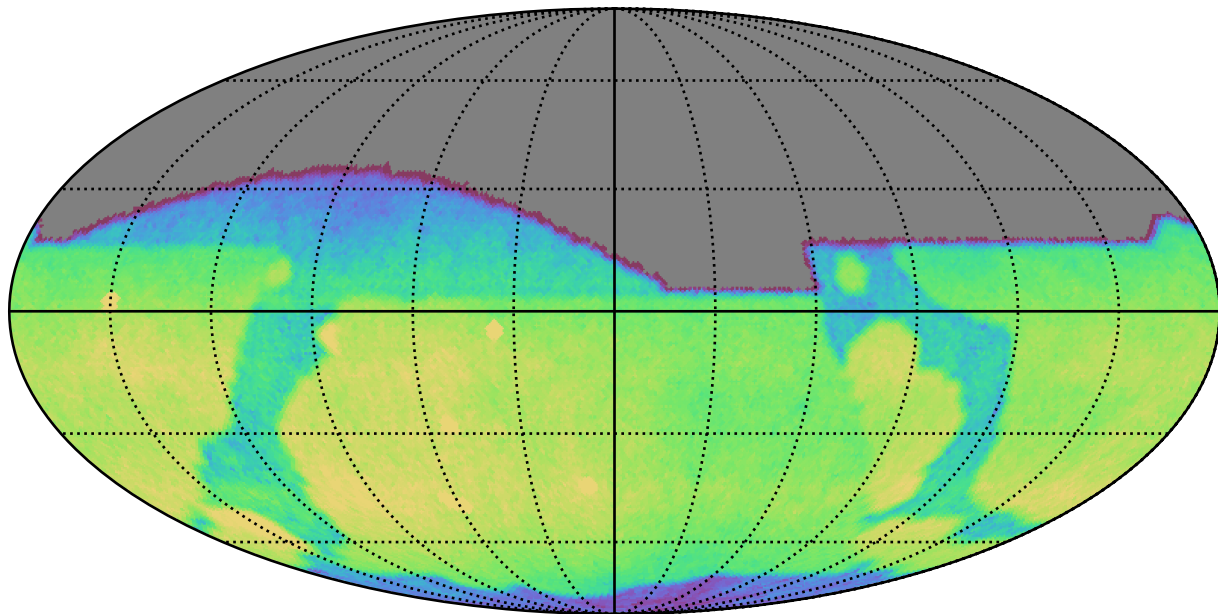
noroll_mjdp120_v3.4_10yrs All sky g band: CoaddM5
