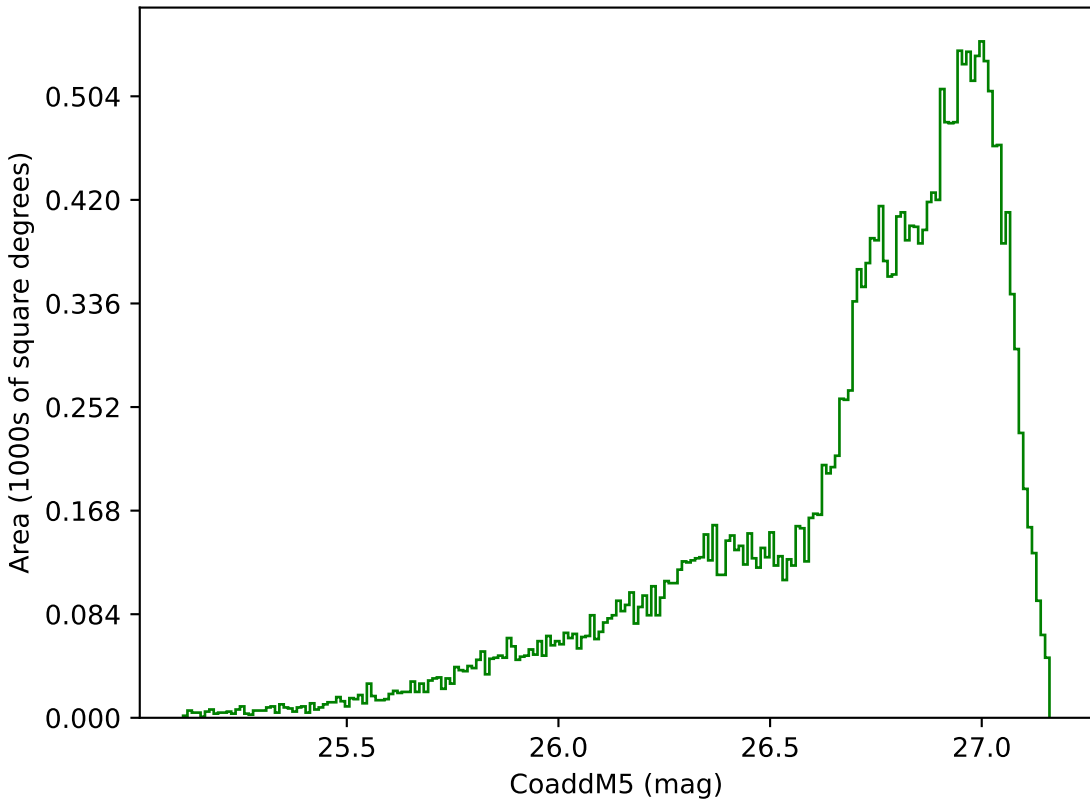
noroll_mjdp120_v3.4_10yrs All sky g band: CoaddM5
