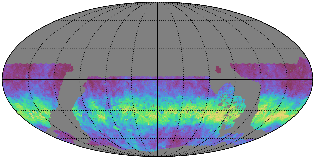
noroll_mjdp120_v3.4_10yrs WFD u band: AngleRms rotSkyPos
