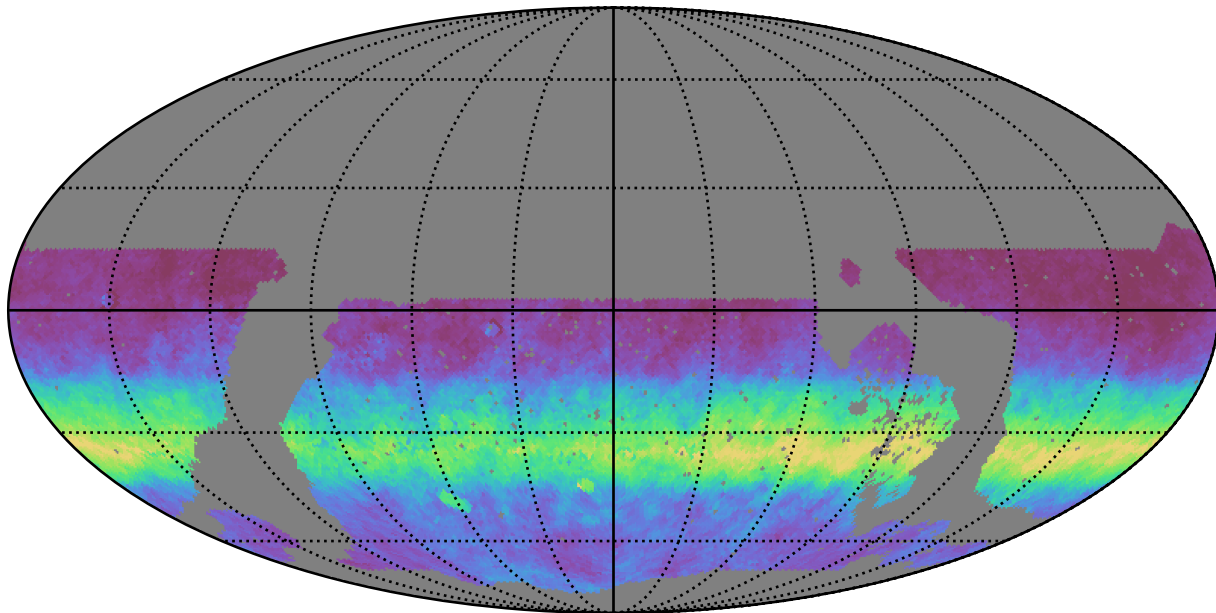
noroll_mjdp120_v3.4_10yrs WFD r band: AngleRms rotSkyPos
