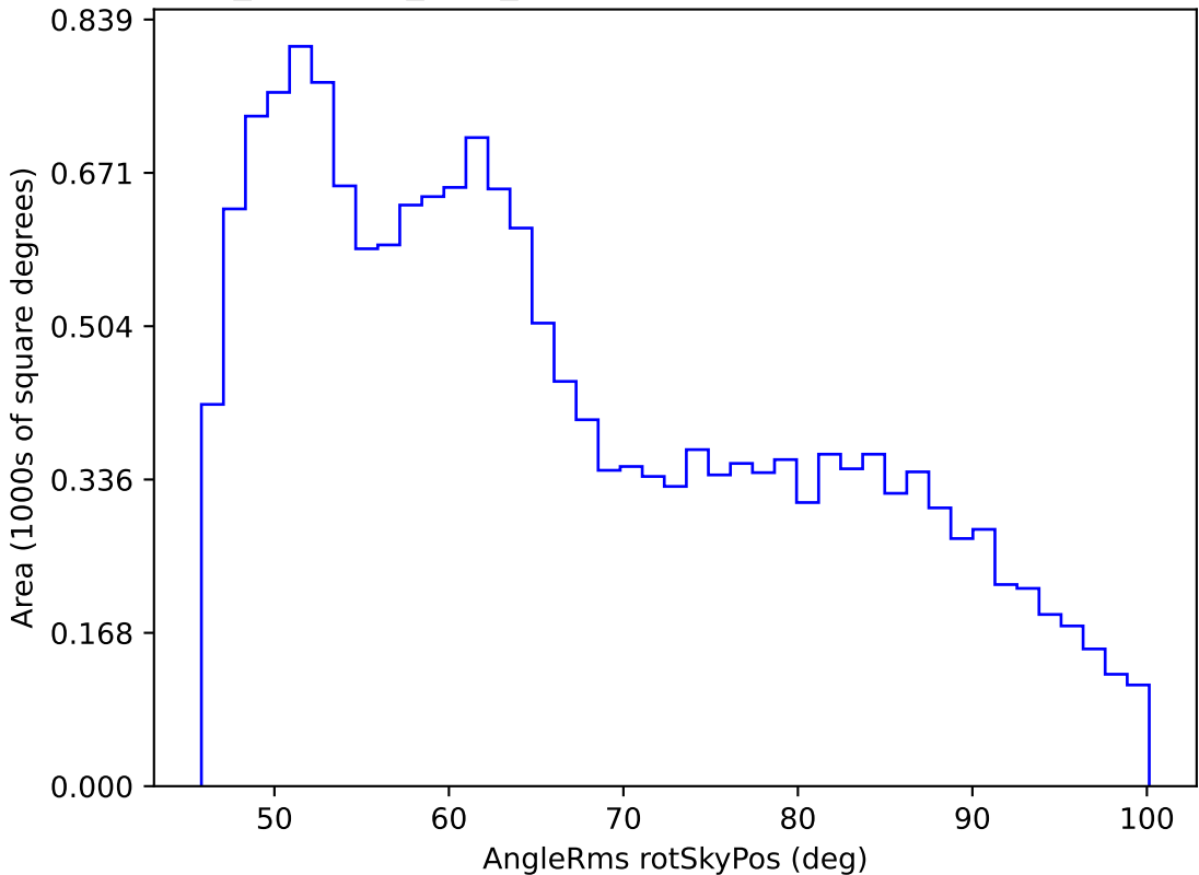
noroll_mjdp120_v3.4_10yrs WFD r band: AngleRms rotSkyPos
