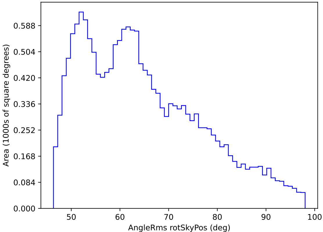
noroll_mjdp120_v3.4_10yrs WFD i band: AngleRms rotSkyPos
