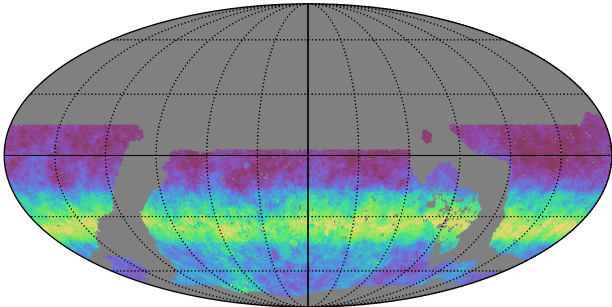
noroll_mjdp120_v3.4_10yrs WFD g band: AngleRms rotSkyPos
