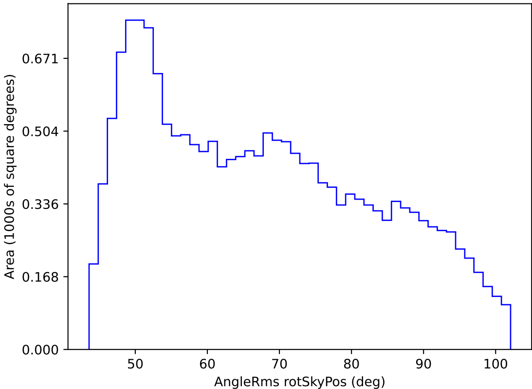
noroll_mjdp120_v3.4_10yrs WFD g band: AngleRms rotSkyPos
