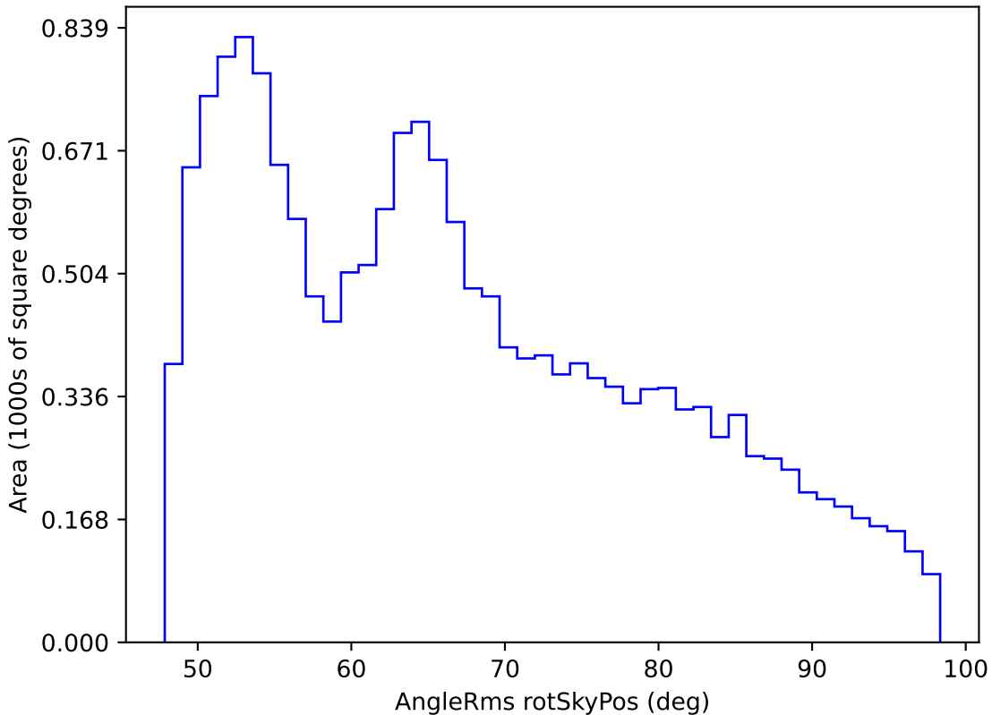
noroll_mjdp120_v3.4_10yrs WFD all bands: AngleRms rotSkyPos
