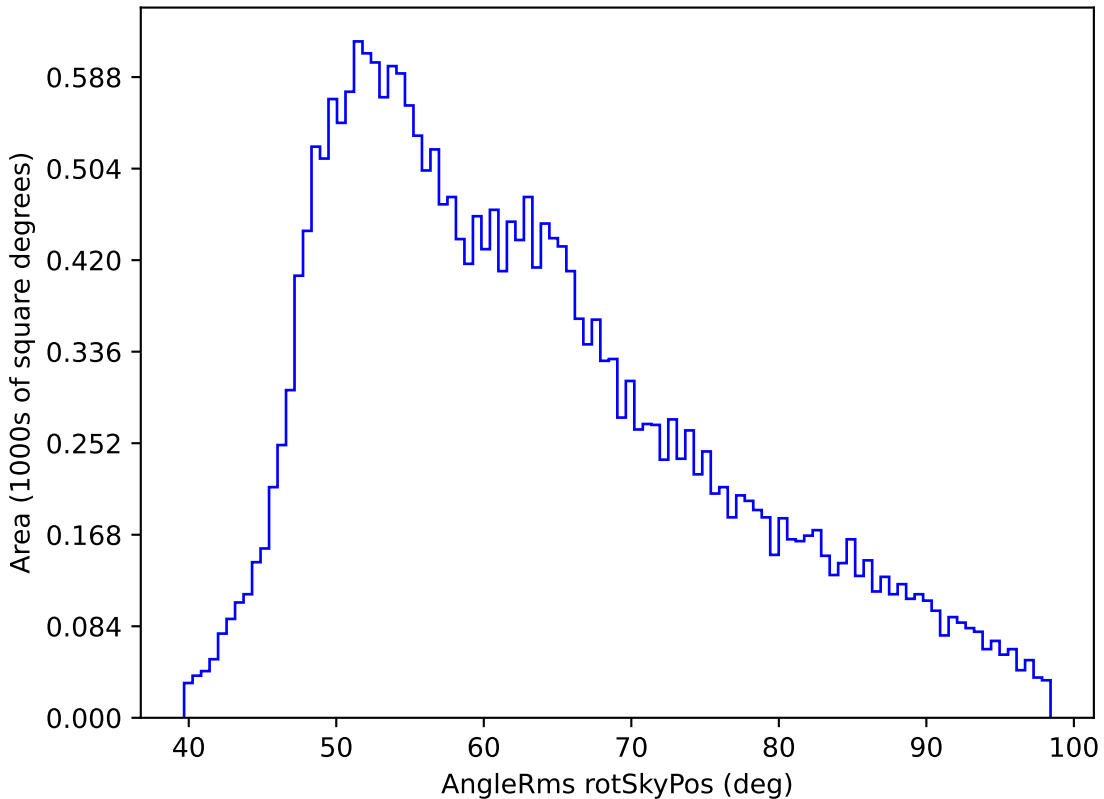
noroll_mjdp120_v3.4_10yrs All sky z band: AngleRms rotSkyPos
