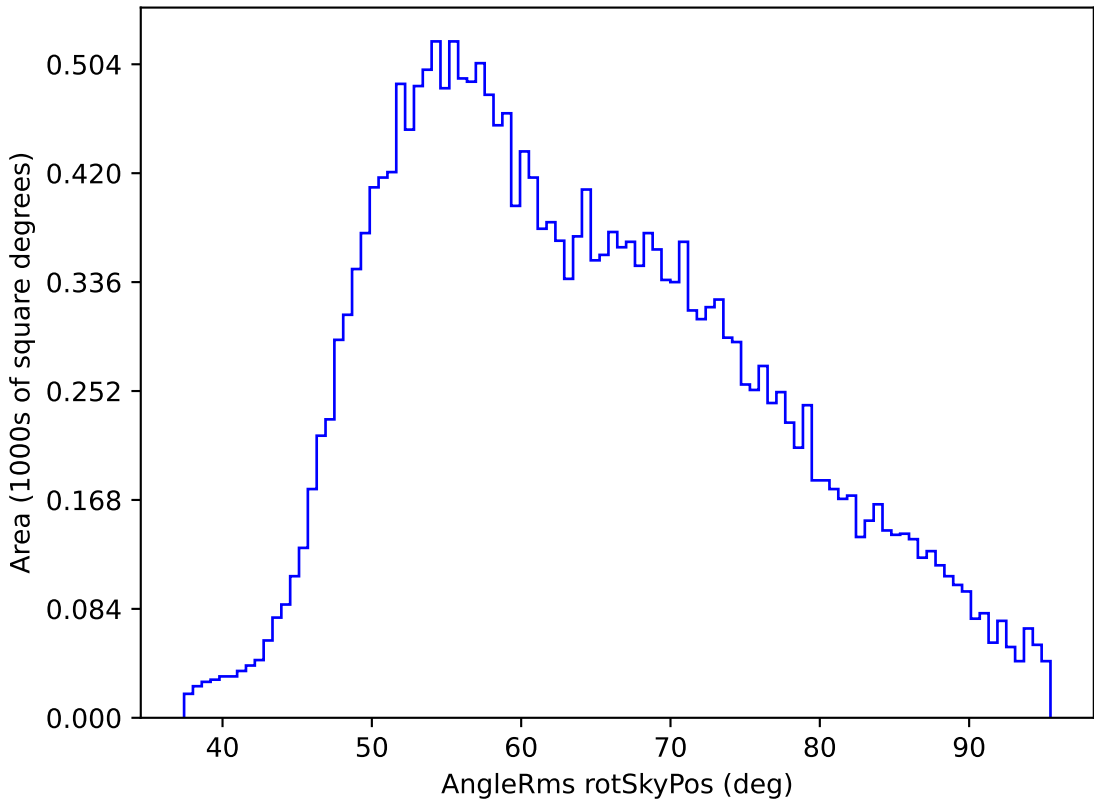
noroll_mjdp120_v3.4_10yrs All sky y band: AngleRms rotSkyPos
