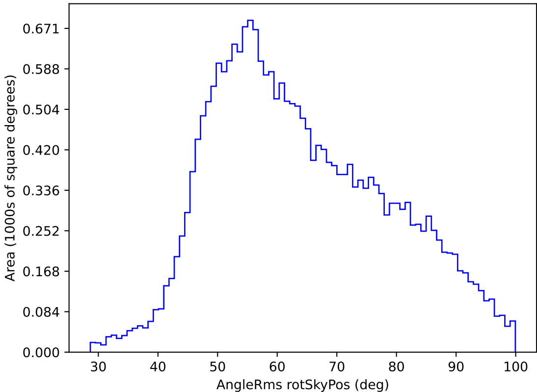
noroll_mjdp120_v3.4_10yrs All sky u band: AngleRms rotSkyPos
