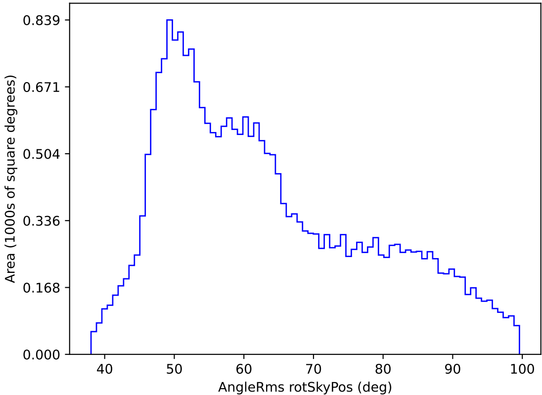
noroll_mjdp120_v3.4_10yrs All sky r band: AngleRms rotSkyPos
