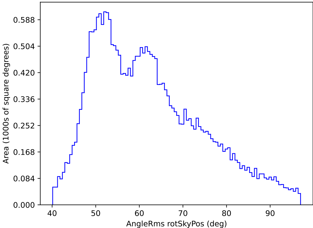
noroll_mjdp120_v3.4_10yrs All sky i band: AngleRms rotSkyPos
