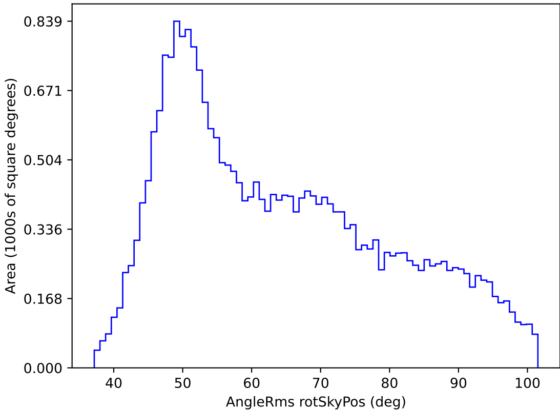
noroll_mjdp120_v3.4_10yrs All sky g band: AngleRms rotSkyPos
