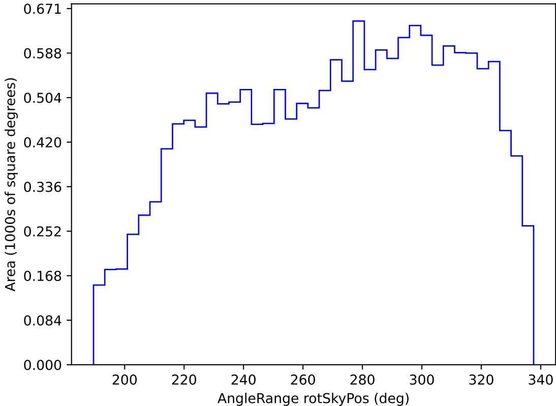
noroll_mjdp120_v3.4_10yrs WFD y band: AngleRange rotSkyPos
