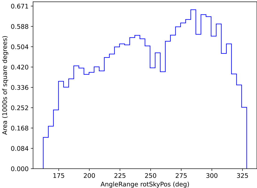
noroll_mjdp120_v3.4_10yrs WFD u band: AngleRange rotSkyPos
