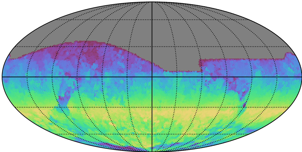
noroll_mjdp120_v3.4_10yrs All sky z band: AngleRange rotSkyPos
