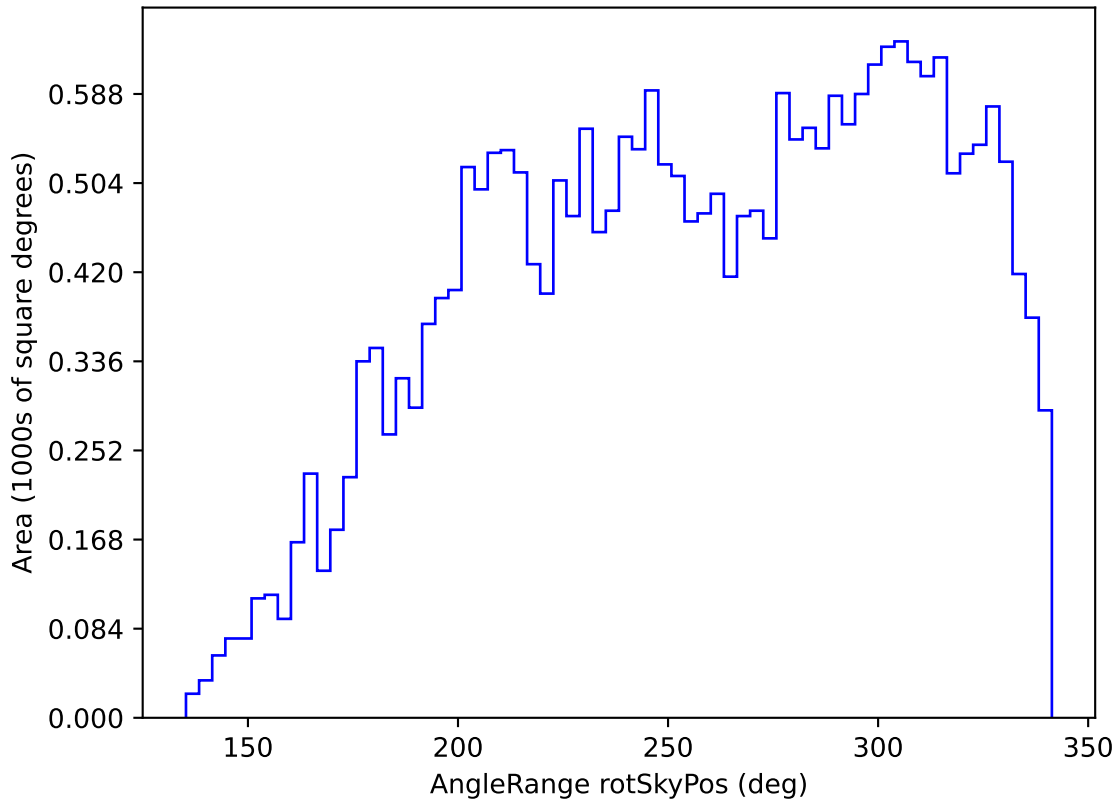
noroll_mjdp120_v3.4_10yrs All sky z band: AngleRange rotSkyPos
