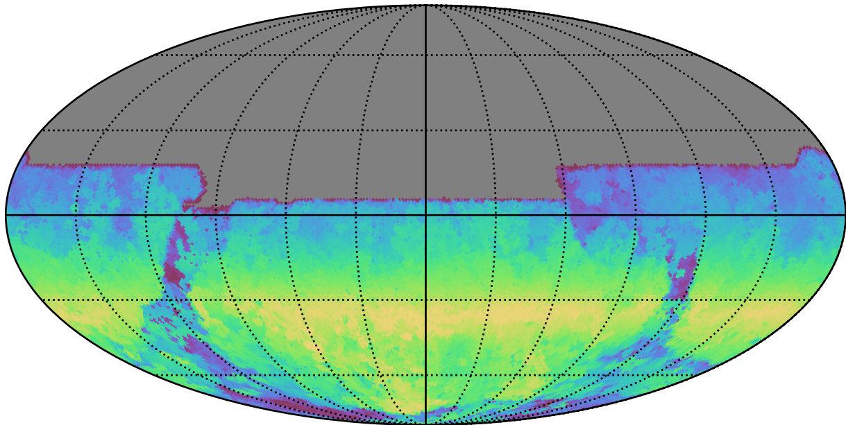
noroll_mjdp120_v3.4_10yrs All sky y band: AngleRange rotSkyPos
