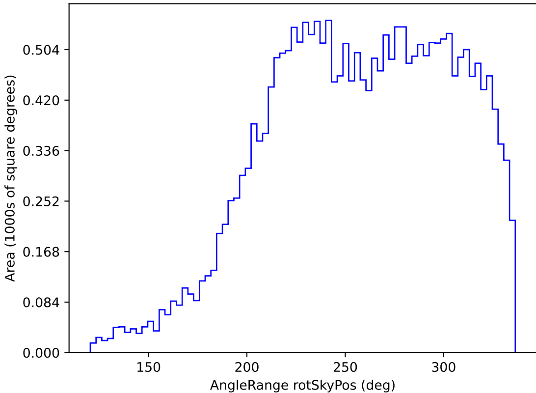
noroll_mjdp120_v3.4_10yrs All sky y band: AngleRange rotSkyPos
