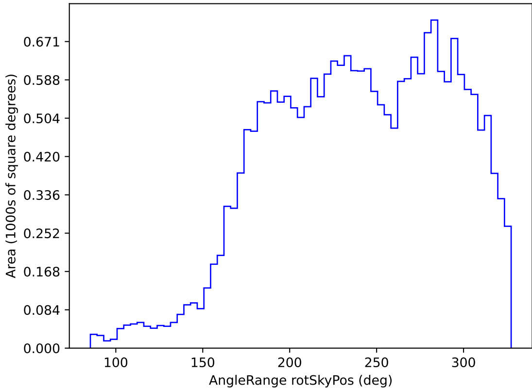
noroll_mjdp120_v3.4_10yrs All sky u band: AngleRange rotSkyPos
