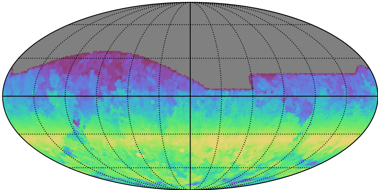
noroll_mjdp120_v3.4_10yrs All sky i band: AngleRange rotSkyPos
