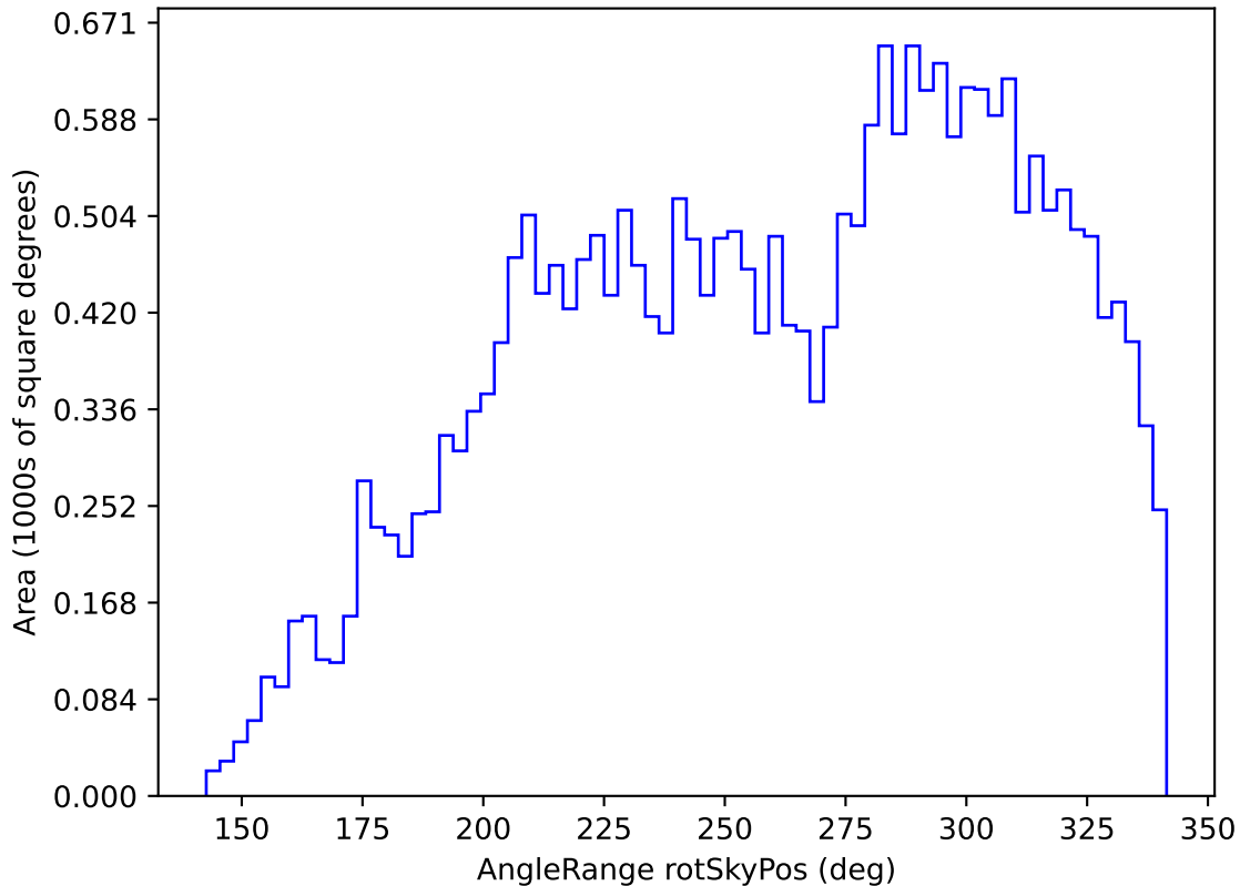
noroll_mjdp120_v3.4_10yrs All sky i band: AngleRange rotSkyPos
