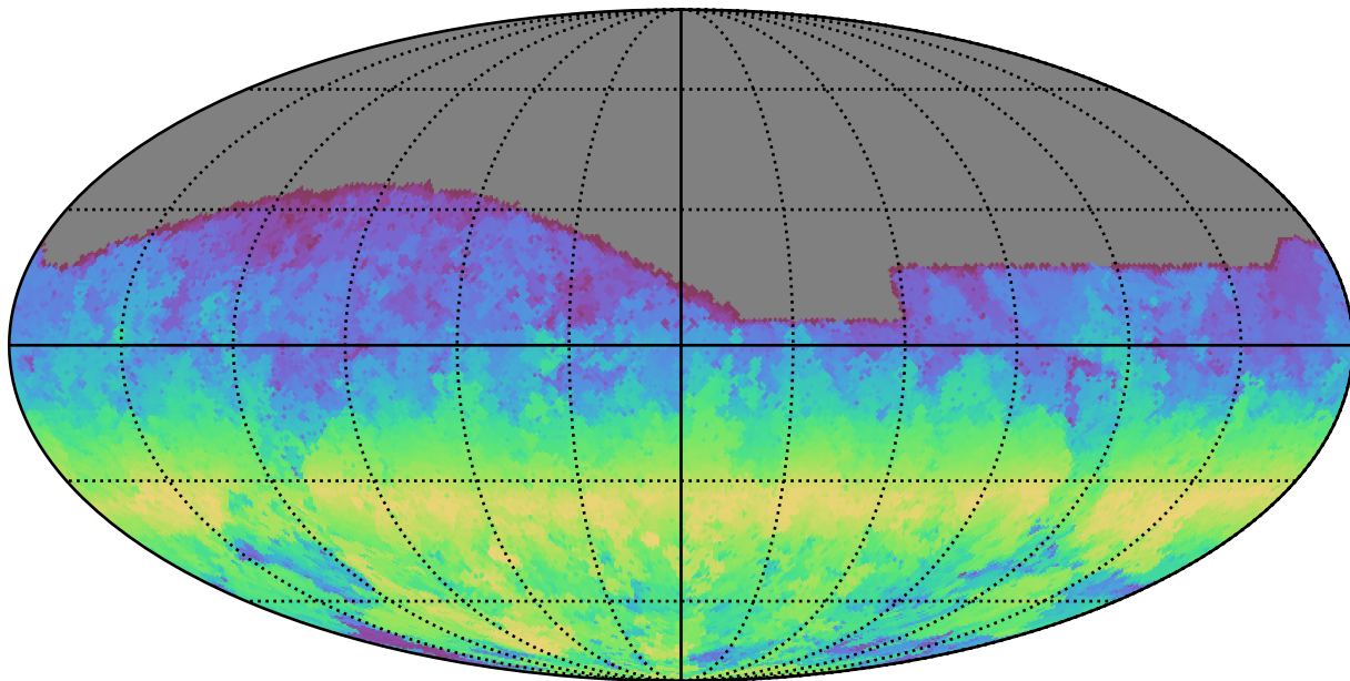
noroll_mjdp120_v3.4_10yrs All sky g band: AngleRange rotSkyPos
