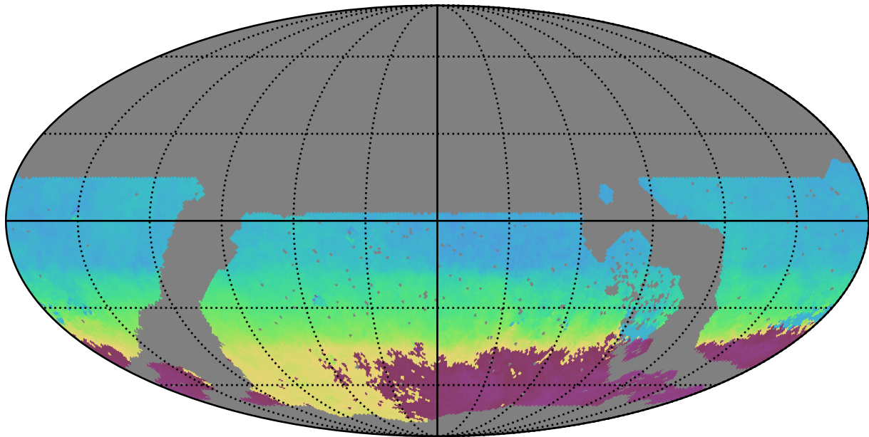
noroll_mjdp120_v3.4_10yrs WFD z band: AngleMean rotSkyPos
