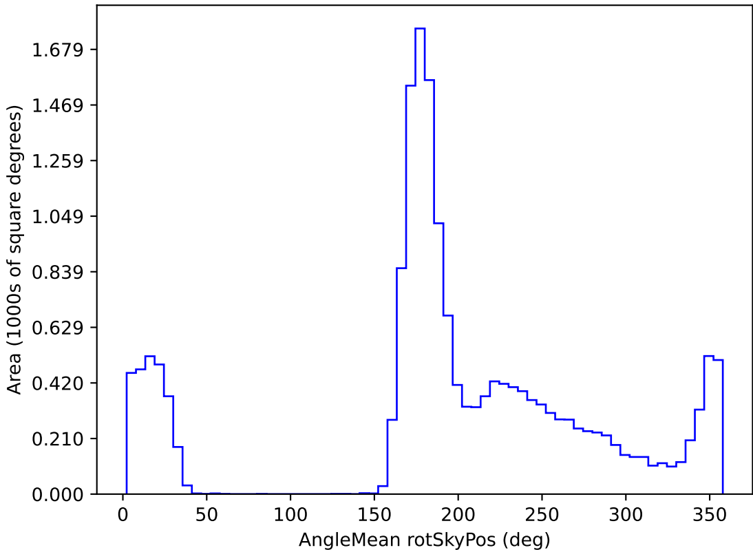
noroll_mjdp120_v3.4_10yrs WFD z band: AngleMean rotSkyPos
