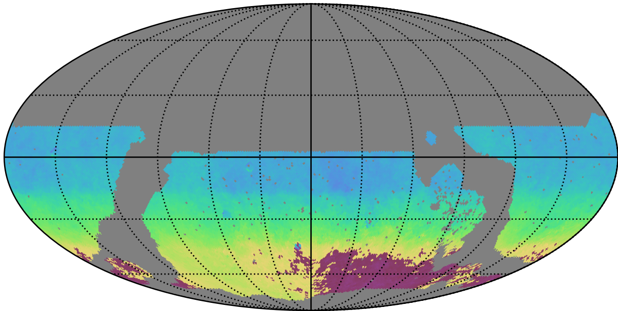
noroll_mjdp120_v3.4_10yrs WFD y band: AngleMean rotSkyPos
