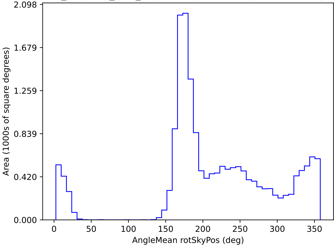
noroll_mjdp120_v3.4_10yrs WFD y band: AngleMean rotSkyPos
