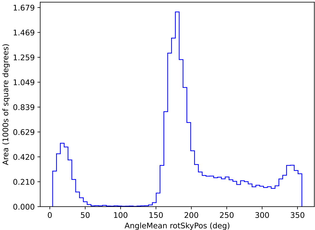
noroll_mjdp120_v3.4_10yrs WFD u band: AngleMean rotSkyPos
