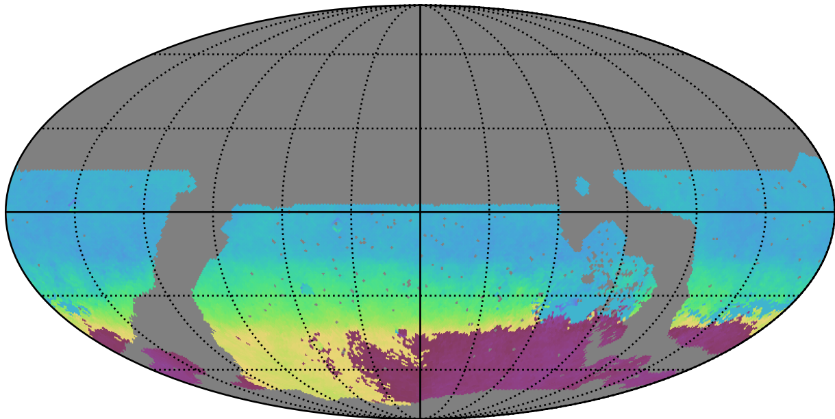
noroll_mjdp120_v3.4_10yrs WFD r band: AngleMean rotSkyPos
