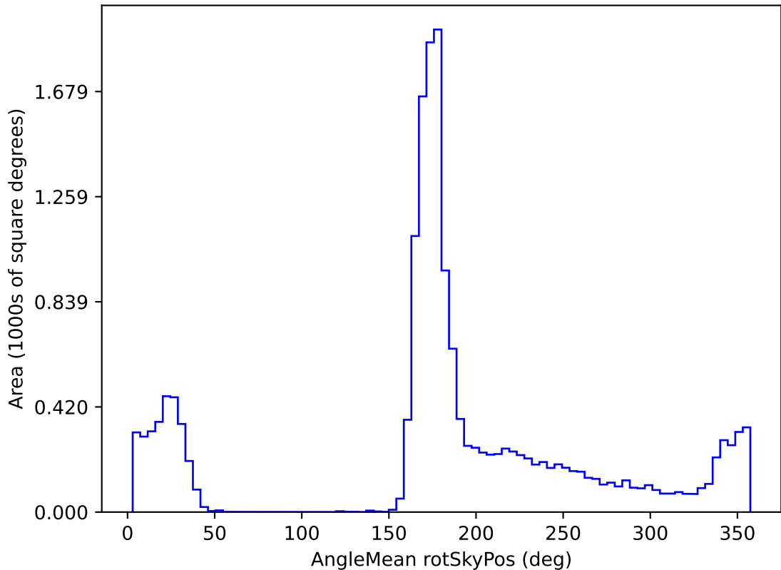
noroll_mjdp120_v3.4_10yrs WFD r band: AngleMean rotSkyPos
