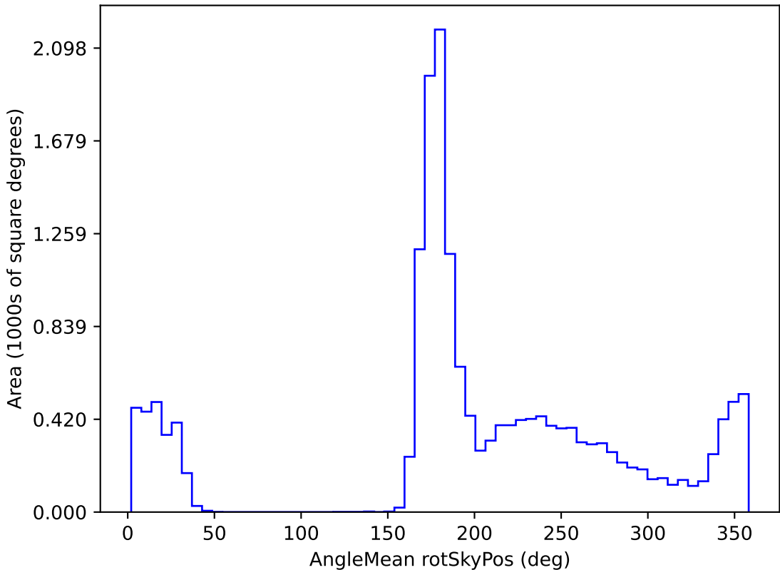
noroll_mjdp120_v3.4_10yrs WFD i band: AngleMean rotSkyPos
