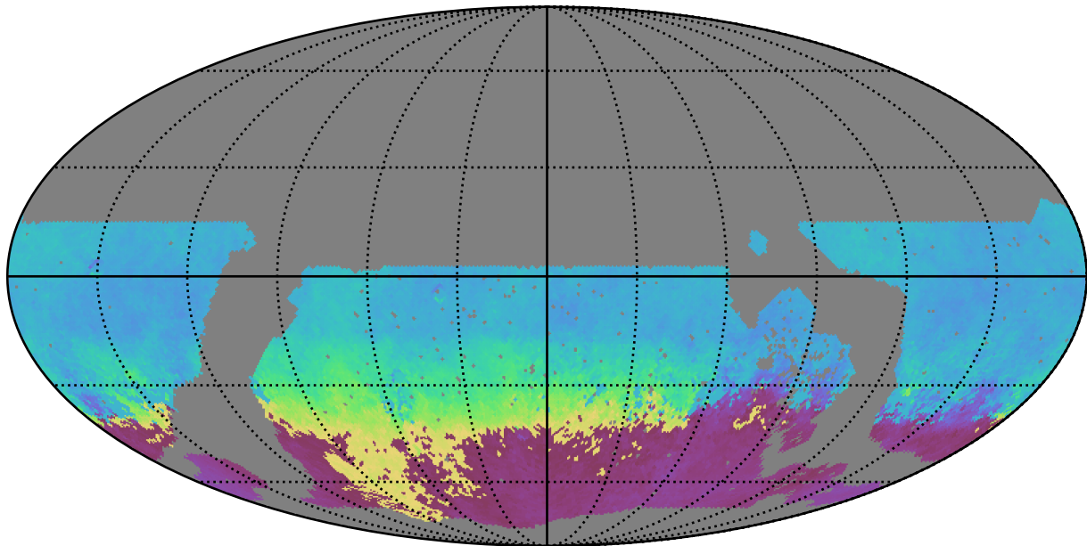
noroll_mjdp120_v3.4_10yrs WFD g band: AngleMean rotSkyPos
