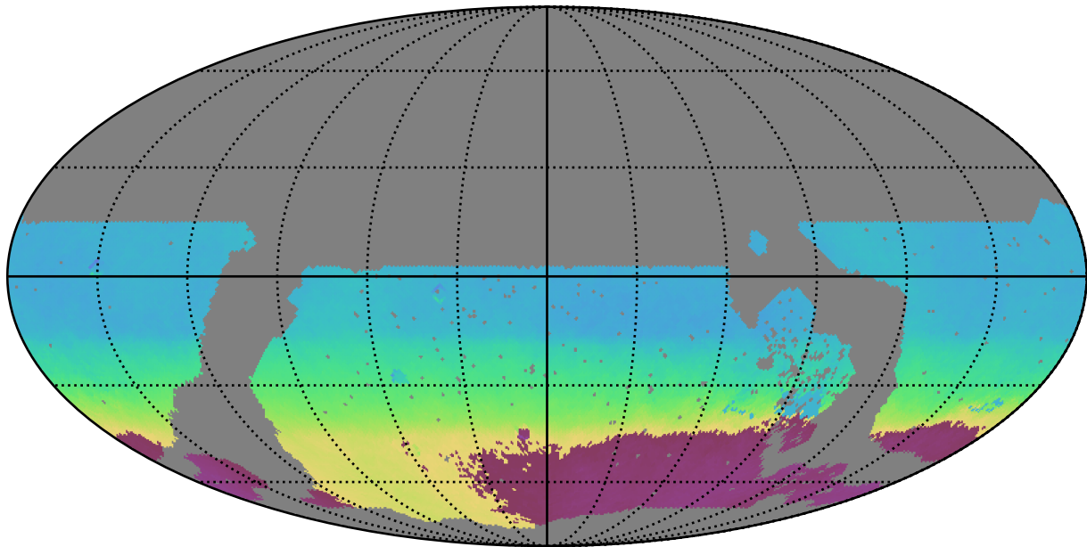
noroll_mjdp120_v3.4_10yrs WFD all bands: AngleMean rotSkyPos
