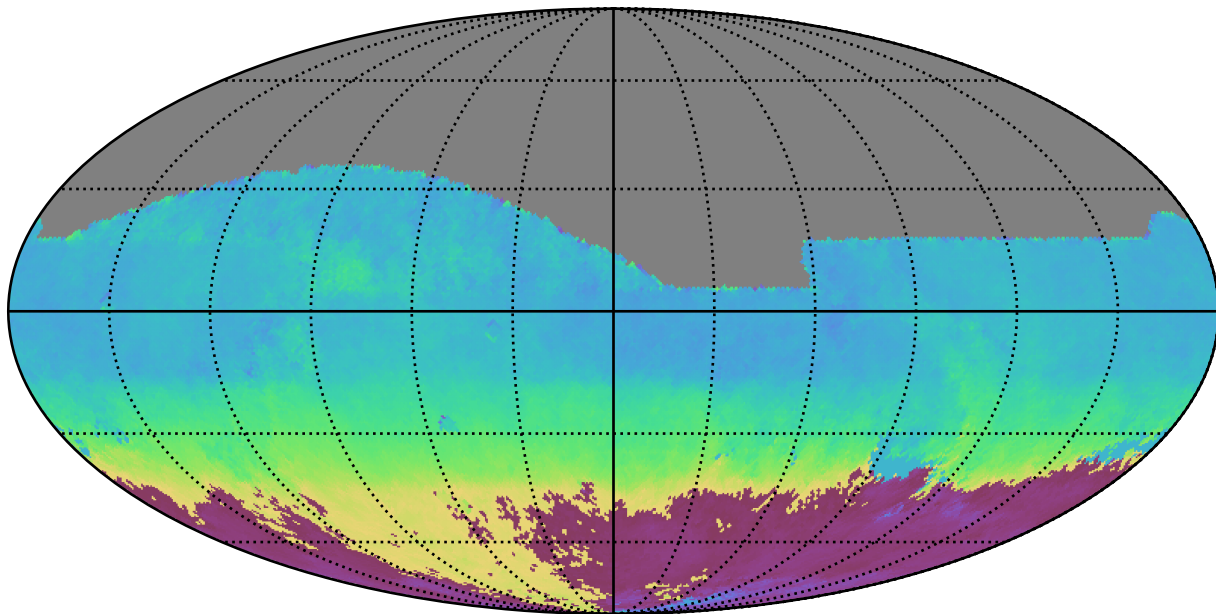
noroll_mjdp120_v3.4_10yrs All sky z band: AngleMean rotSkyPos
