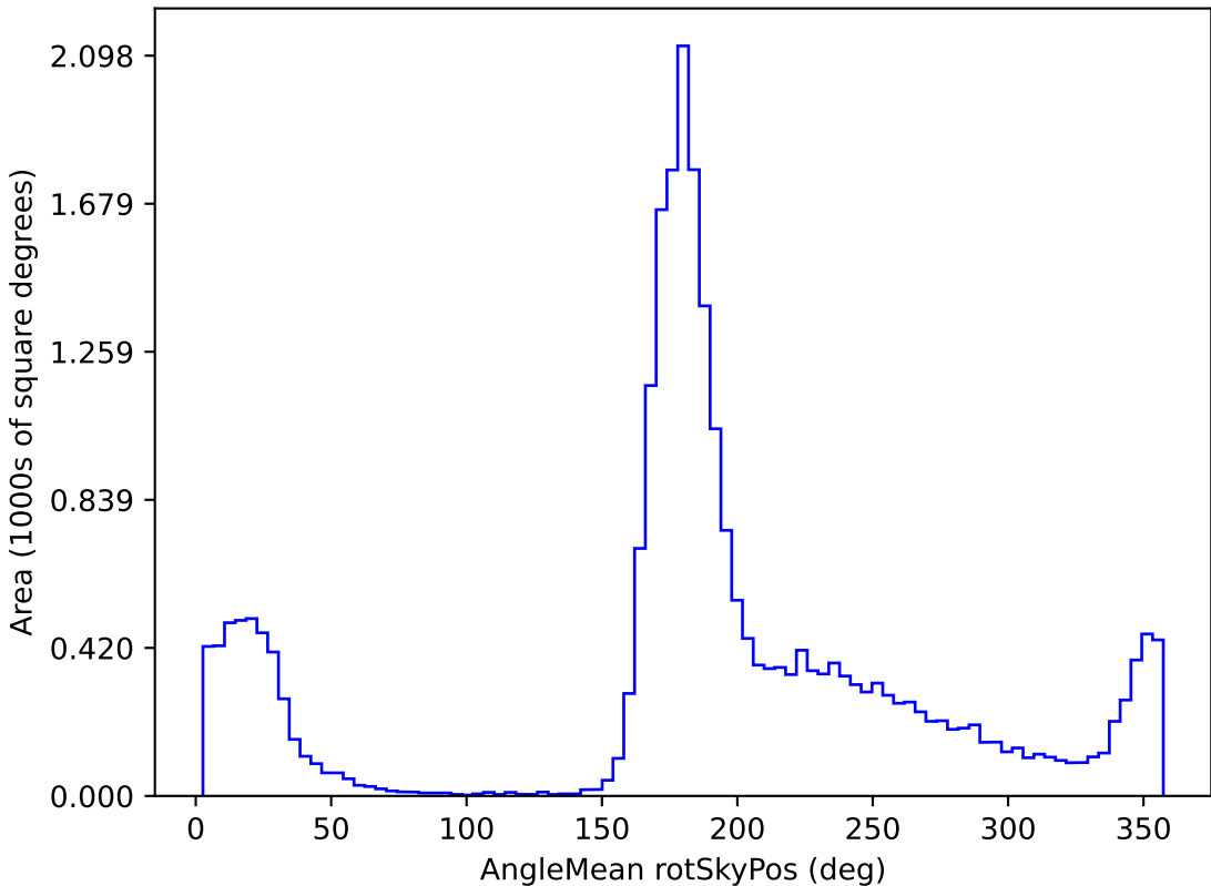
noroll_mjdp120_v3.4_10yrs All sky z band: AngleMean rotSkyPos
