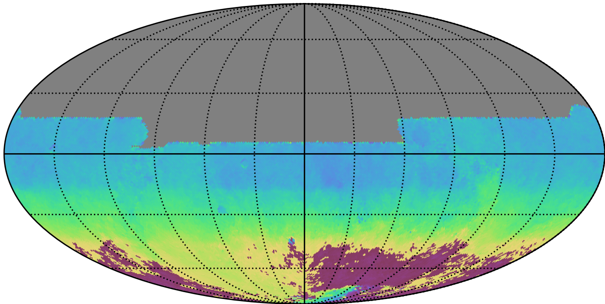
noroll_mjdp120_v3.4_10yrs All sky y band: AngleMean rotSkyPos
