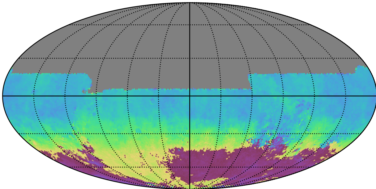
noroll_mjdp120_v3.4_10yrs All sky u band: AngleMean rotSkyPos
