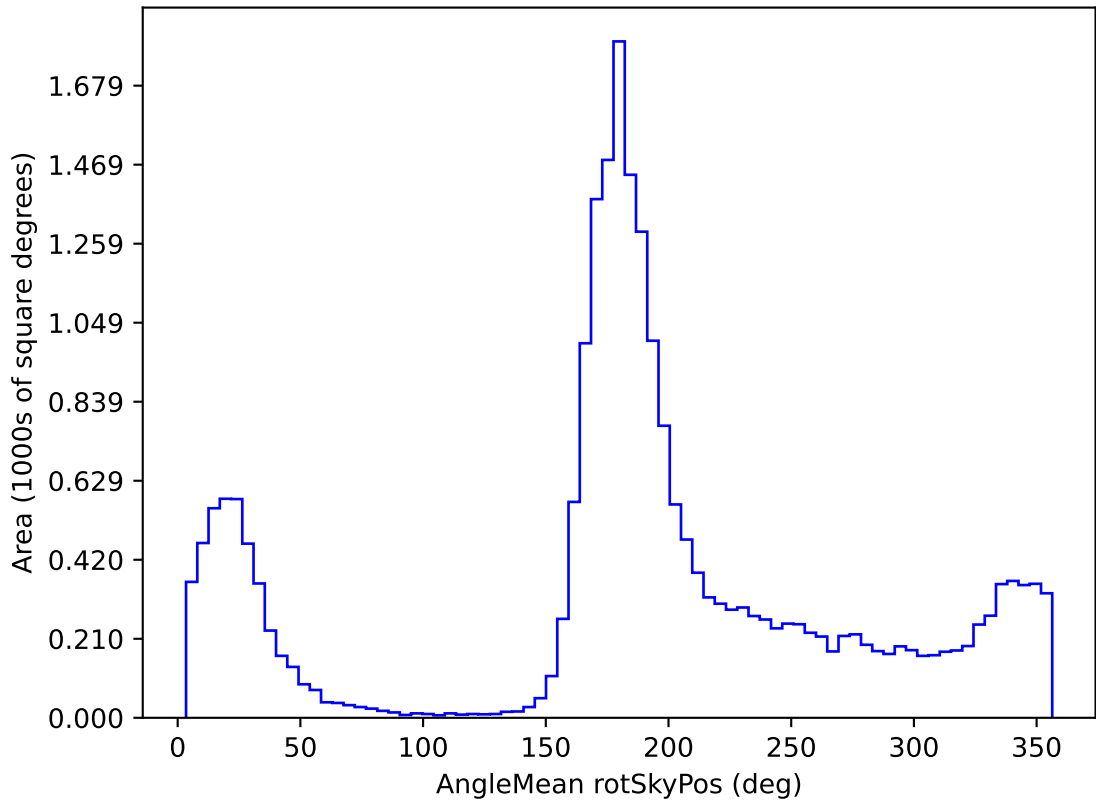
noroll_mjdp120_v3.4_10yrs All sky u band: AngleMean rotSkyPos
