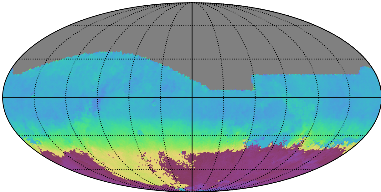
noroll_mjdp120_v3.4_10yrs All sky r band: AngleMean rotSkyPos
