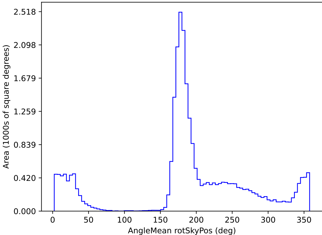
noroll_mjdp120_v3.4_10yrs All sky i band: AngleMean rotSkyPos
