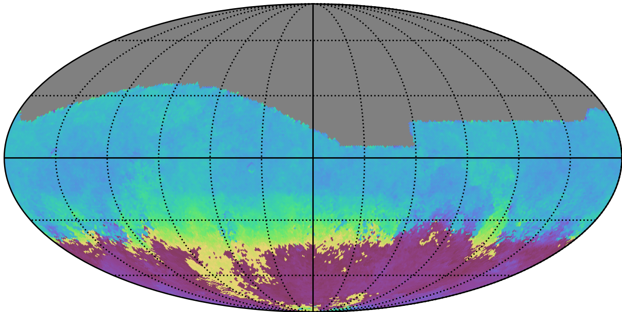
noroll_mjdp120_v3.4_10yrs All sky g band: AngleMean rotSkyPos
