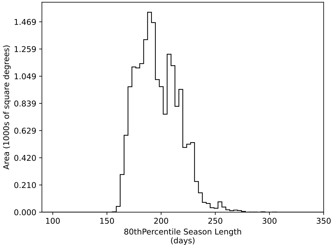
noroll_mjdp120_v3.4_10yrs WFD all bands: 80thPercentile Season Length
