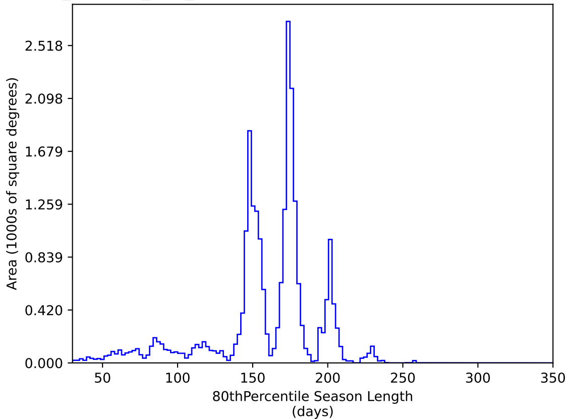
noroll_mjdp120_v3.4_10yrs All sky y band: 80thPercentile Season Length
